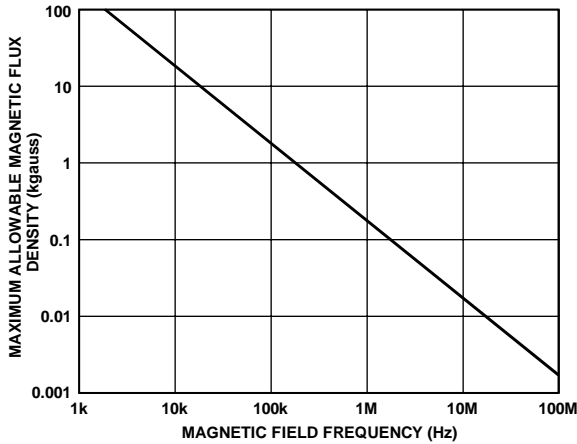
Figure 18. Maximum Allowable External Magnetic Flux Density
